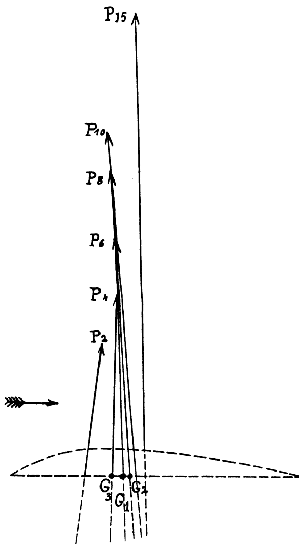
FIG. 89.—Sheaf of total pressures on a complete Bleriot XI. monoplane.
